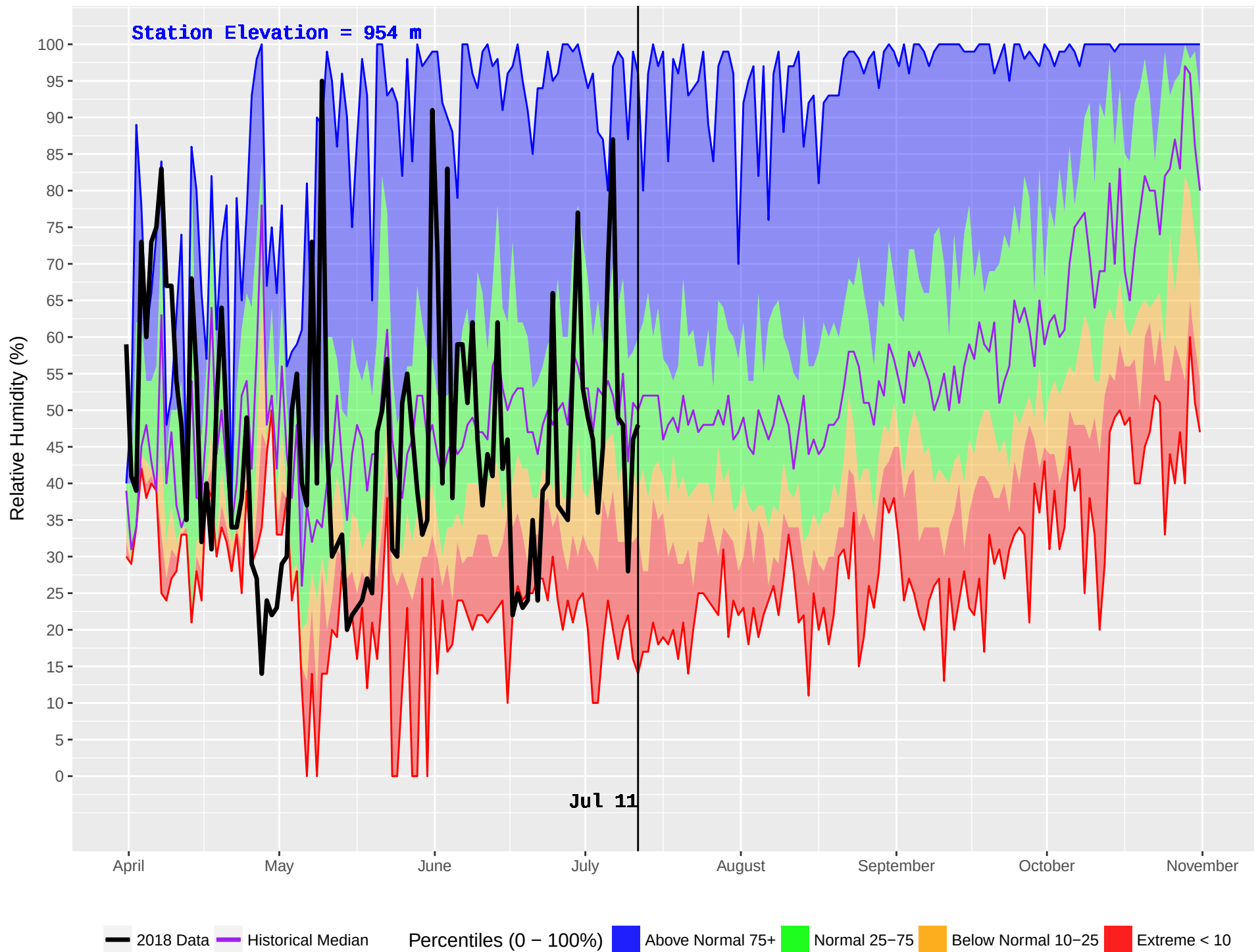
NADINA (179) : Historical (1985–2016) and Current (2018) Noon Relative Humidity
